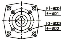
PNEUMATIC ACTUATOR
