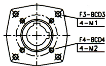
VALVE MOUNTING
